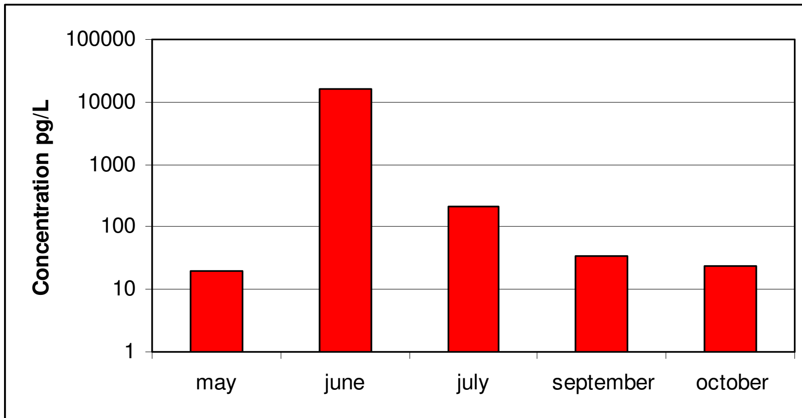
Figure 4. Trend of concentrations of total PCBs in the Frodolfo stream in spring-autumn 2006
