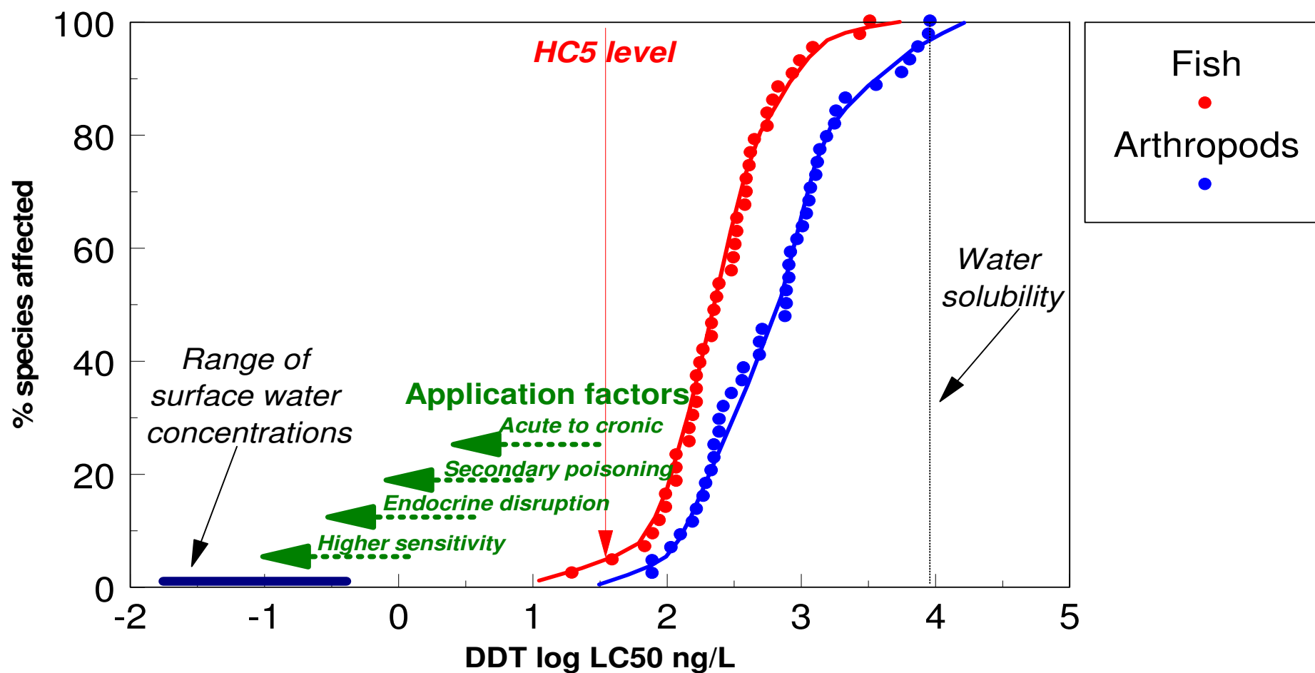
Figure 5. SSD curves for DDT compared with DDT concentrations measured in glacial streams. To estimate a safe concentration, HC5 should be reduced through a series of application factors (explanation in the text).
