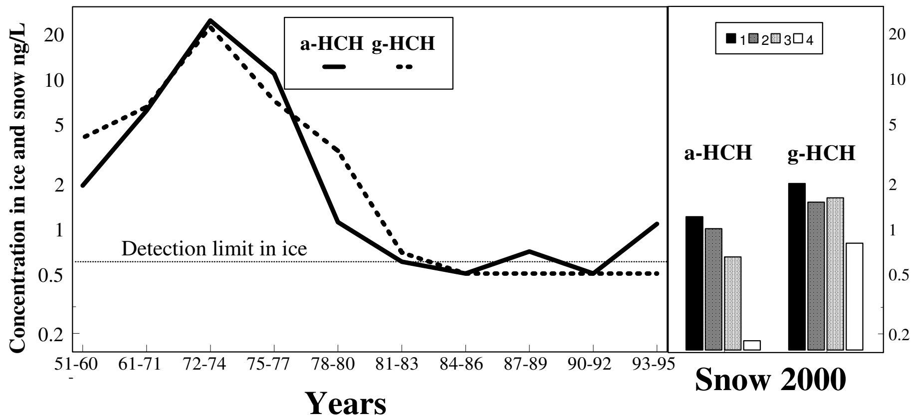
Figure 1. Concentrations of HCHs in the different layers of the Lys glacier ice core, corresponding to a time span from 1950 to 1996, and in new (1) and aged (2 to 4) snow samples collected in June 2000 (modified after Villa et. al. , 2003).
